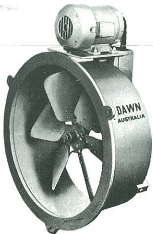
Enclosed Propellers . . 5 sizes 450 mm to 1200 mm Open Propellers . . . . 5 sizes 450 mm to 1200 mm Split-Hub Propellers . . 5 sizes 625 mm to 1200 mm
