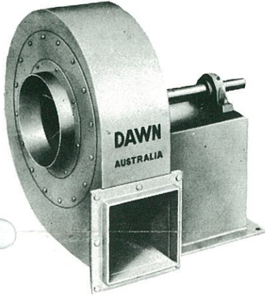
Mill Exhausts . . . . . 8 sizes 225 mm to 600 mm
